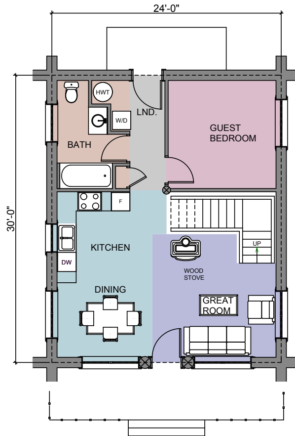
FIRST FLOOR PLAN AREA: 747 SQ.FT.
