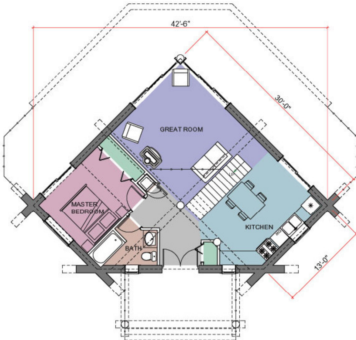
FIRST FLOOR PLAN AREA: 762 SQ. FT.
