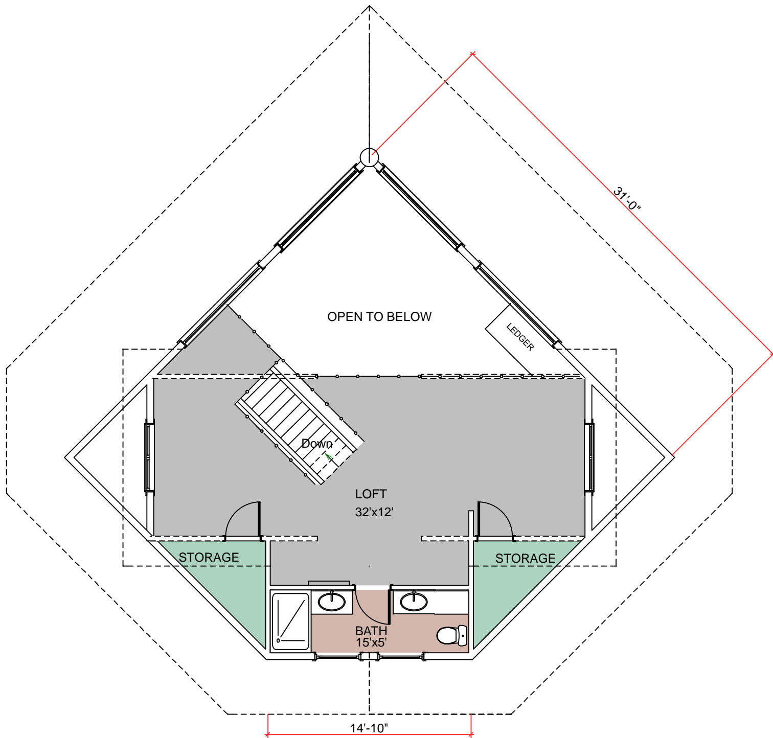
SECOND FLOOR PLAN AREA: 522 SQ. FT.
